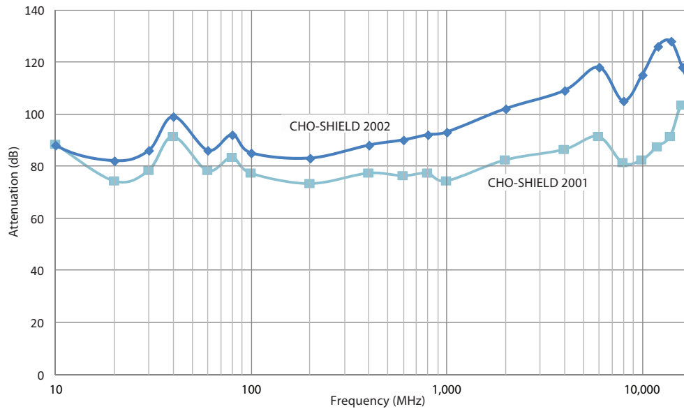
Figure 2: Shielding Effectiveness*
